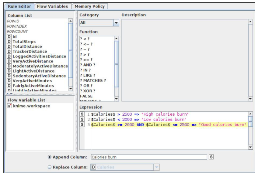
Figure 5: Configuration of Rule Engine node
