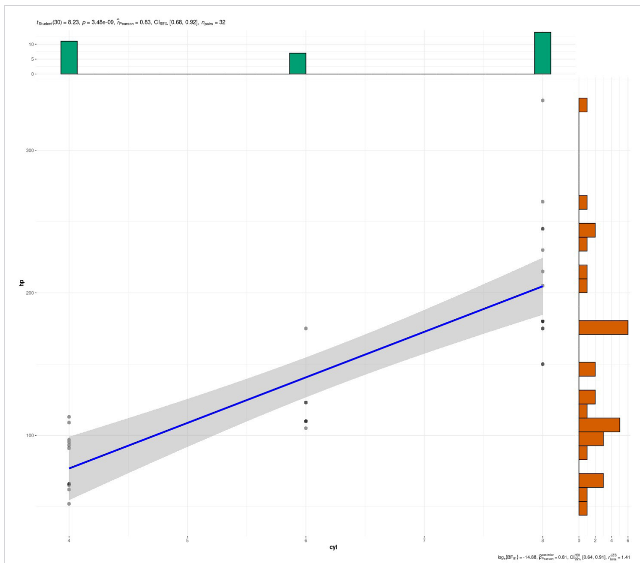
Figure 6: ggscatterstats
