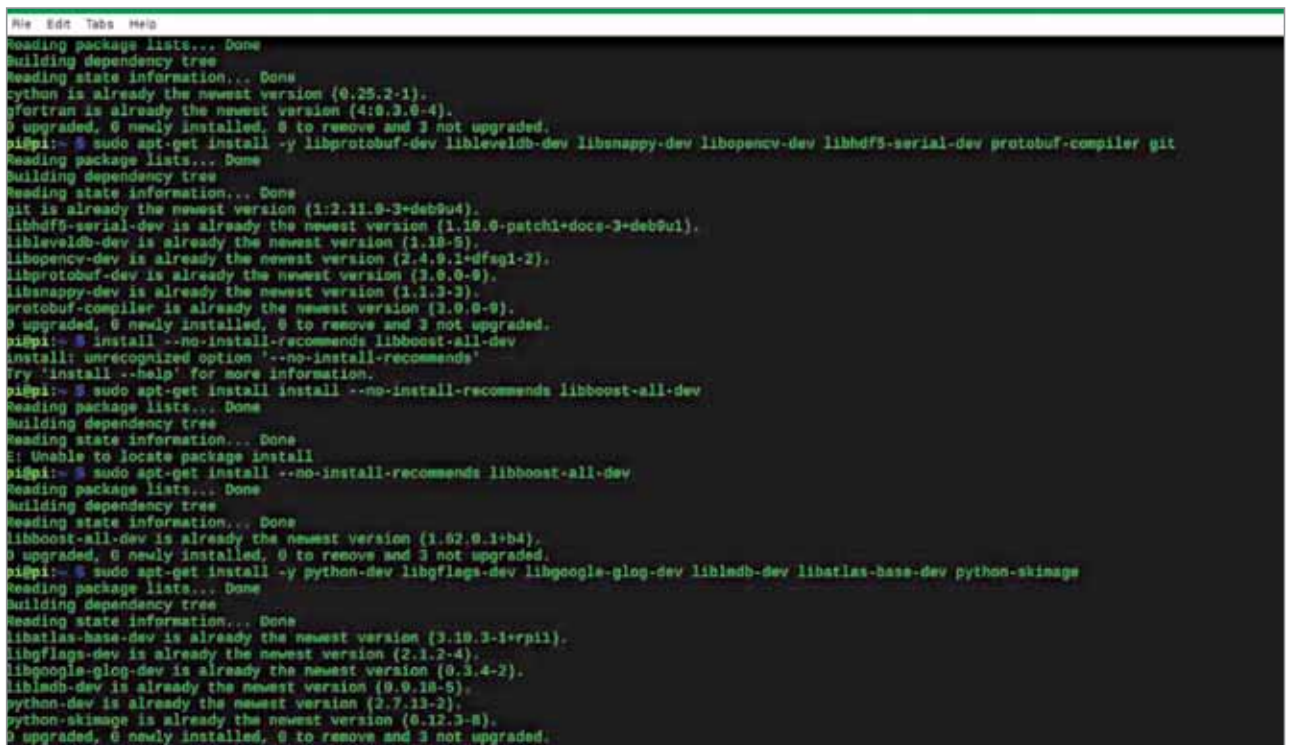
Figure 5: Installing Python modules
