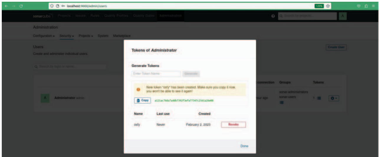
Figure 6: User token
