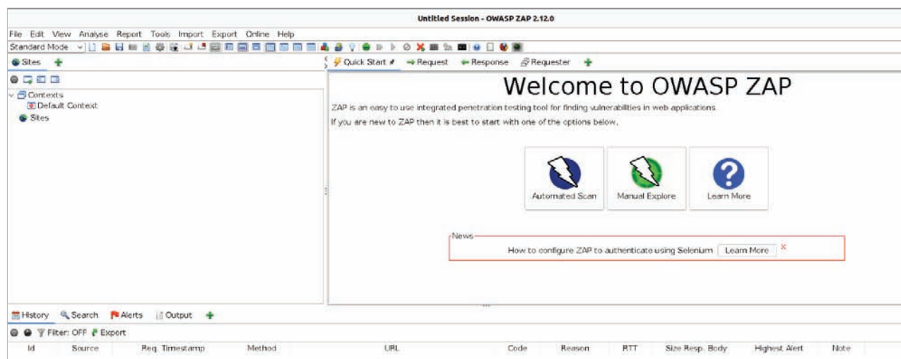
Figure 2: Application in action
