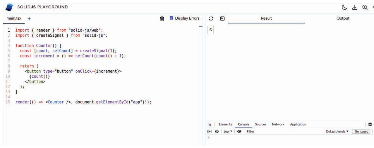
Figure 3: SolidJS playground
