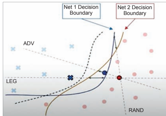
Figure 12: Transfer-based attacks
