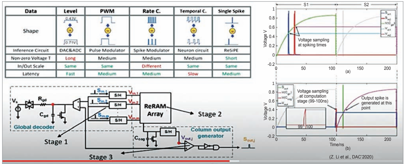
Figure 11: ReRAM based processing engine: ReSiPE
