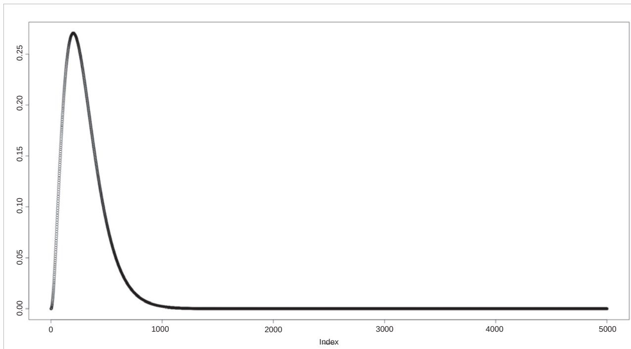
Figure 7: Gamma function
