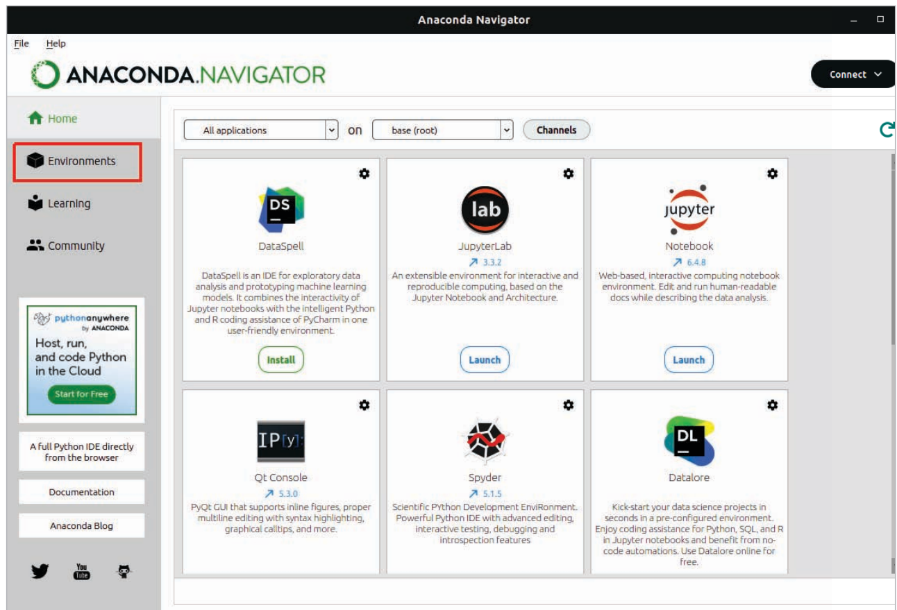
Figure 1: Anaconda Navigator
