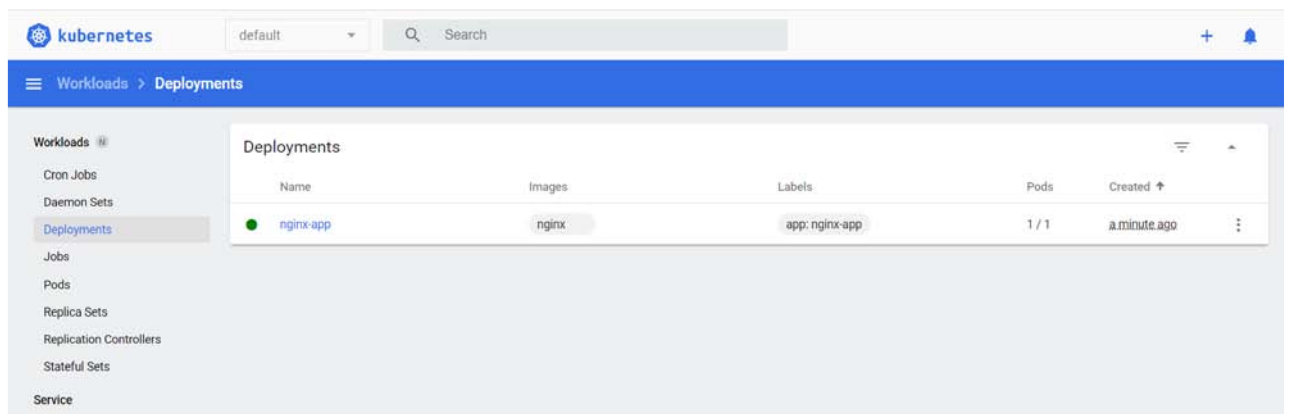
Figure 5: Nginx deployment
