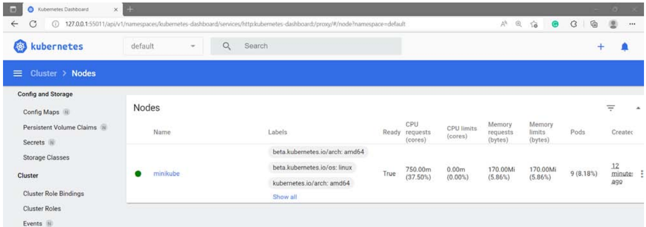
Figure 3: Minikube dashboard
