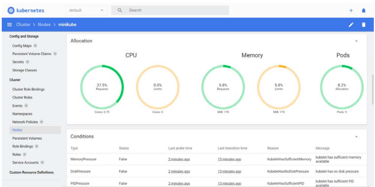
Figure 4: Minikube resources
