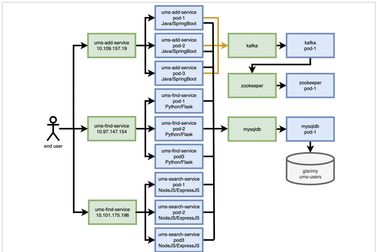
Figure 3: UMS deployment architecture
