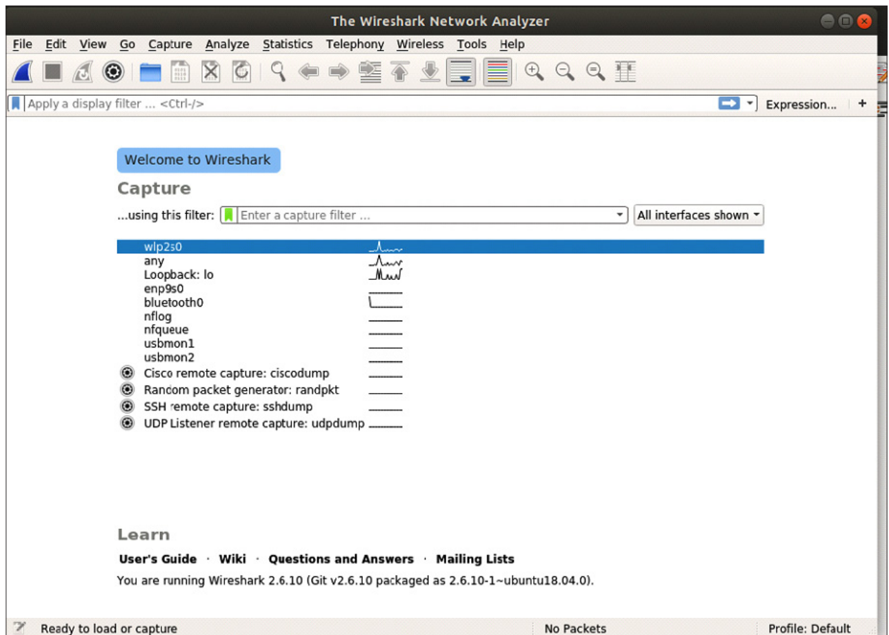
Figure 2: Wireshark window
