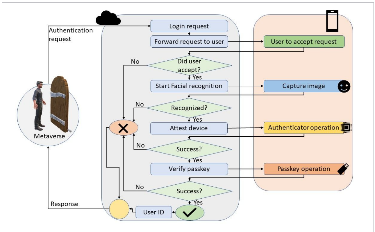
Figure 2: Workflow of MetaKey
