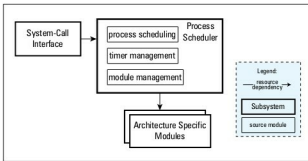
Figure 2: Process scheduler structure
