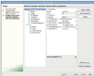
Figure 7: Add-in Wizard: Function properties
