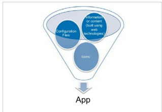
Figure 2: App structure
