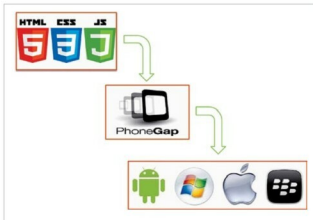
Figure 1: PhoneGap's structure
