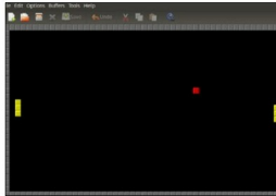
Figure 2: Pong
