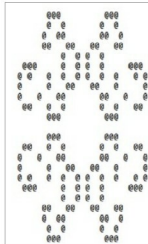
Figure 4: Conway's Life
