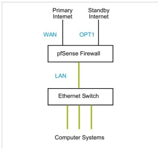
Figure 2: pfSense in dual WAN
