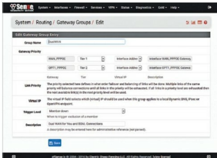
Figure 4: Gateway Group – DualWAN
