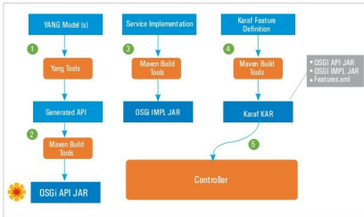
Figure 2: ODL application development workflow
