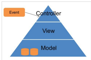
Figure 5: MVC architecture
