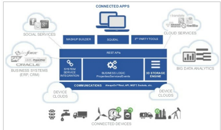
Figure 3: The ThingWorx platform's architecture – Copyright ThingWorx
