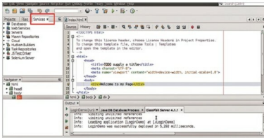
Figure 4: Services tab
