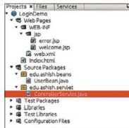
Figure 11: Application structure
