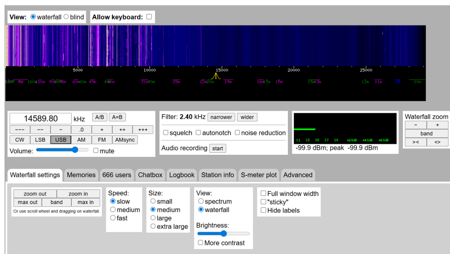
Figure 4: Radio signals analysis and waterfall in cloud KiwiSDR
