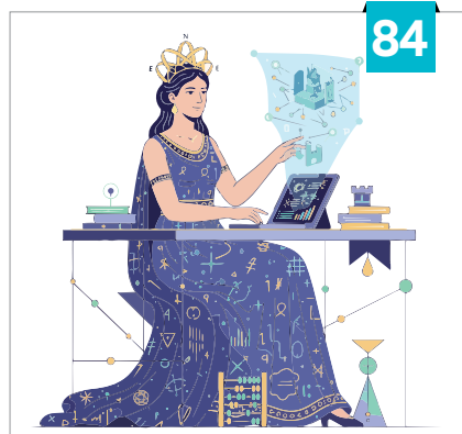
SageMath: Computing with the Queen of Mathematics
