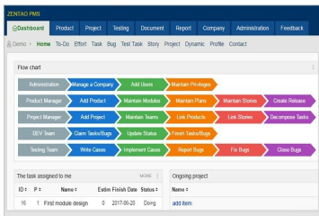
Figure 5: ZenTao user interface
