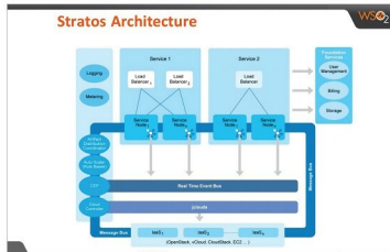
Figure 1: WSO2 architecture (Source: https://wso2.com/platform )
