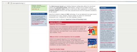
Figure 4: OpenCms
