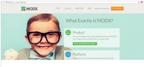
Figure 8: MODX
