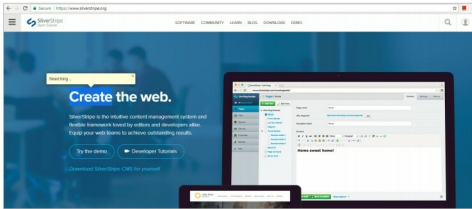
Figure 7: SilverStripe
