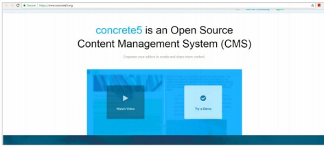
Figure 6: concrete5
