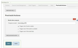
Figure 9: Downstream job
