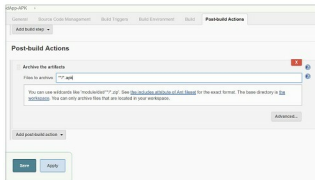
Figure 8: Archive Artifact
