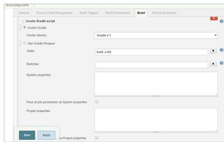
Figure 7: Gradle build
