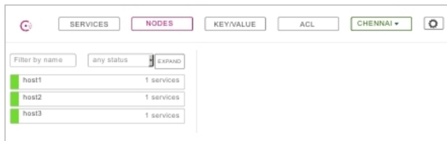
Figure 2: Consul nodes
