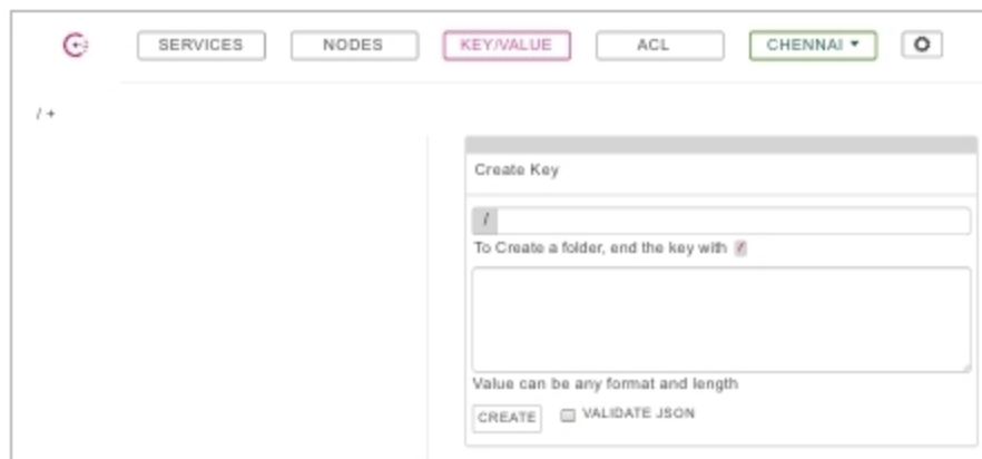
Figure 3: Consul key/value
