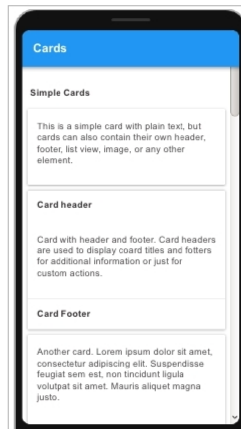
Figure 4: The Card UI component in Framework7
