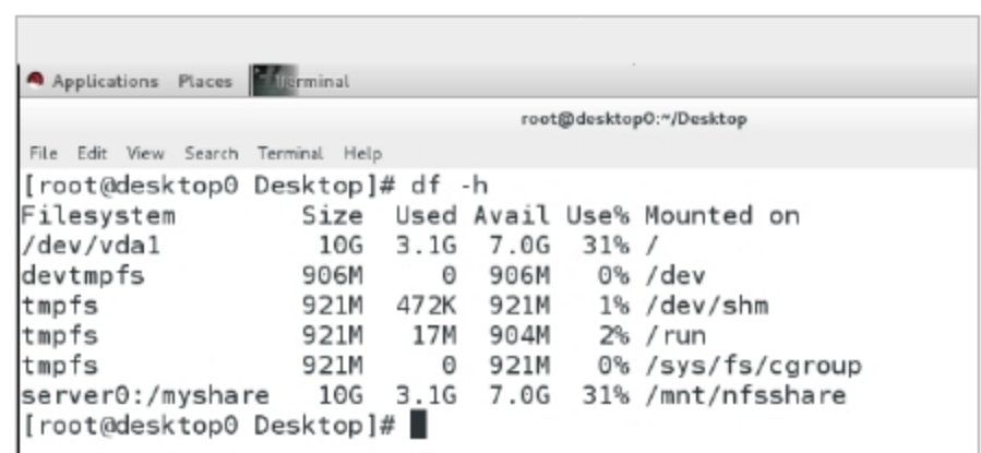
Figure7: Verify the shared directory
