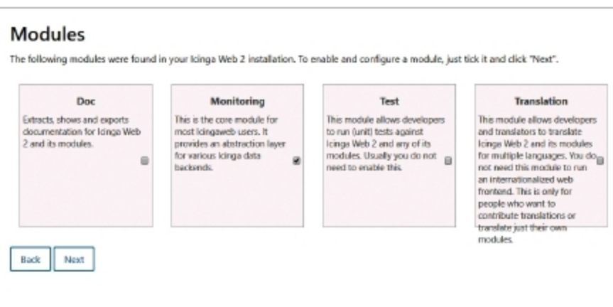
Figure 6: Enabling the monitoring module in the Icinga Web 2 setup
