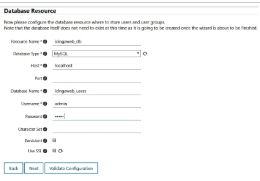
Figure 7: Database configuration details
