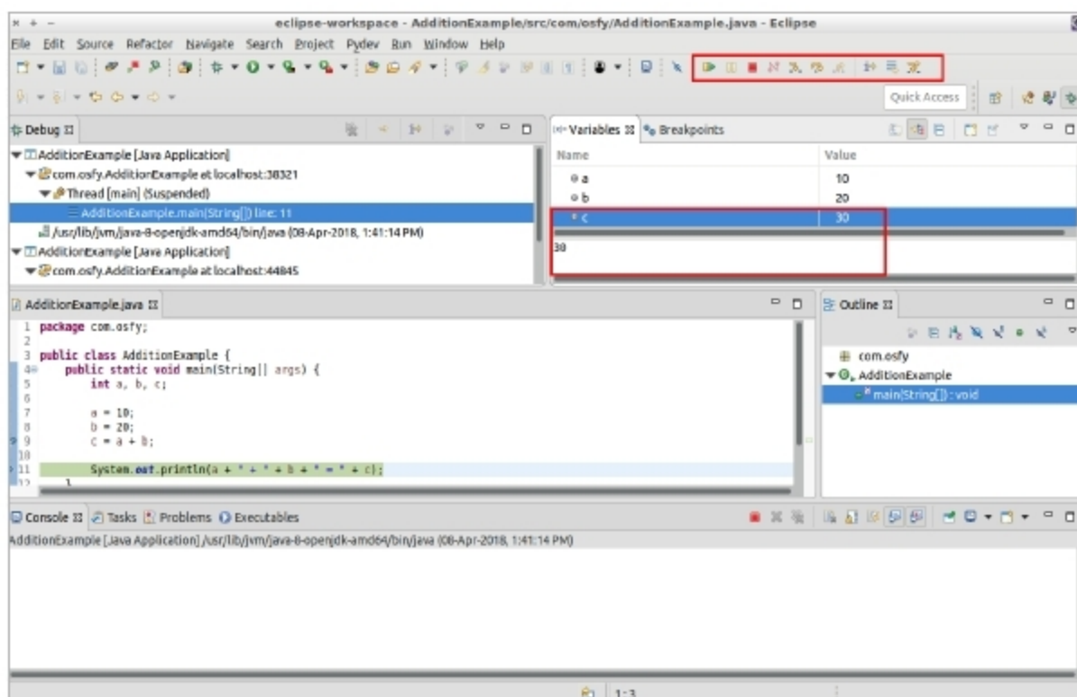
Figure 8: Debugger actions
