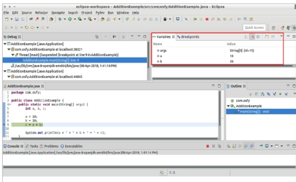
Figure 7: Inspecting variables
