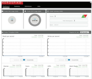
Figure 2: AMC dashboard
