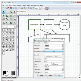
Figure 2: Drawing flowcharts using Dia (Image source: googleimages.com)
