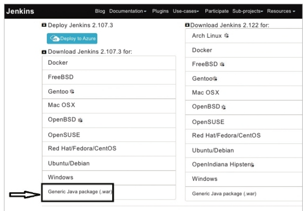
Figure 1: Downloading Jenkins
