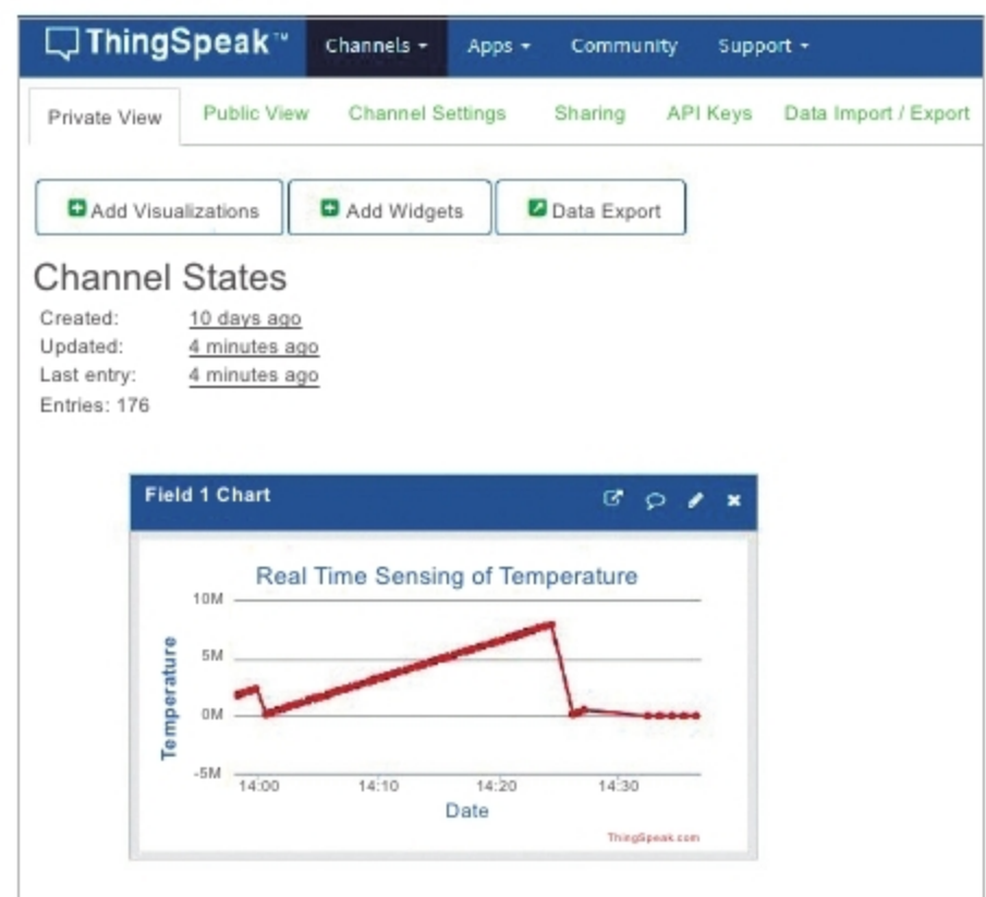
Figure 6: Visualisation of recorded data on ThingSpeak
