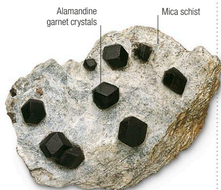
Almandine in matrix | This specimen has a number of classic almandine garnet dodecahedrons embedded in a groundmass of mica schist.
