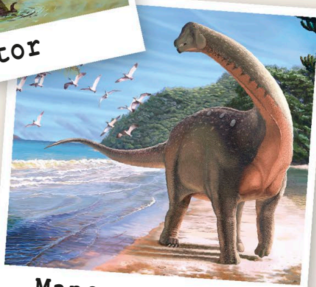
Mansourasaurus
