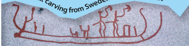
Rock carving from Sweden showing a boat
