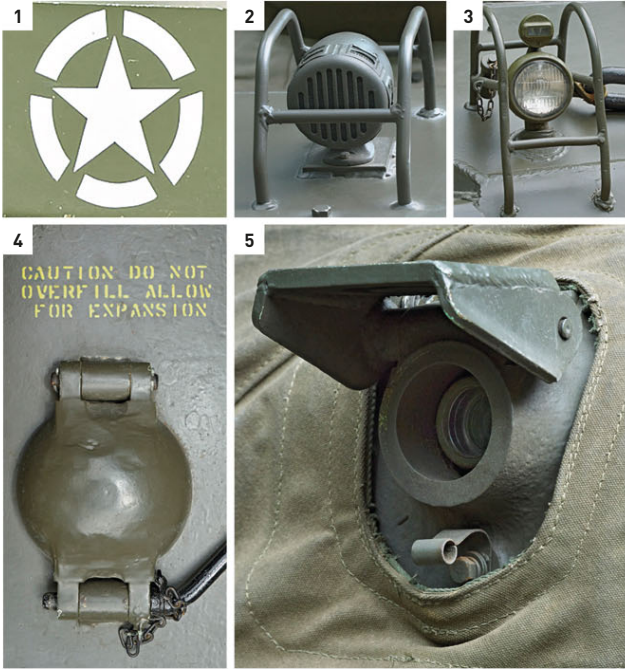
1. Allied recognition symbol 2. Klaxon 3. Headlamp 4. Fuel filler cover 5. Main gunsight aperture 6. Gunner's periscope 7. Commander's machine gun 8. Gun cleaning rods stowed on hull 9. Crewman's stowage 10. Machine gun tripod for ground use 11. Shovel stowed on hull 12. Return roller under top of track 13. Rear light 14. Engine bay
