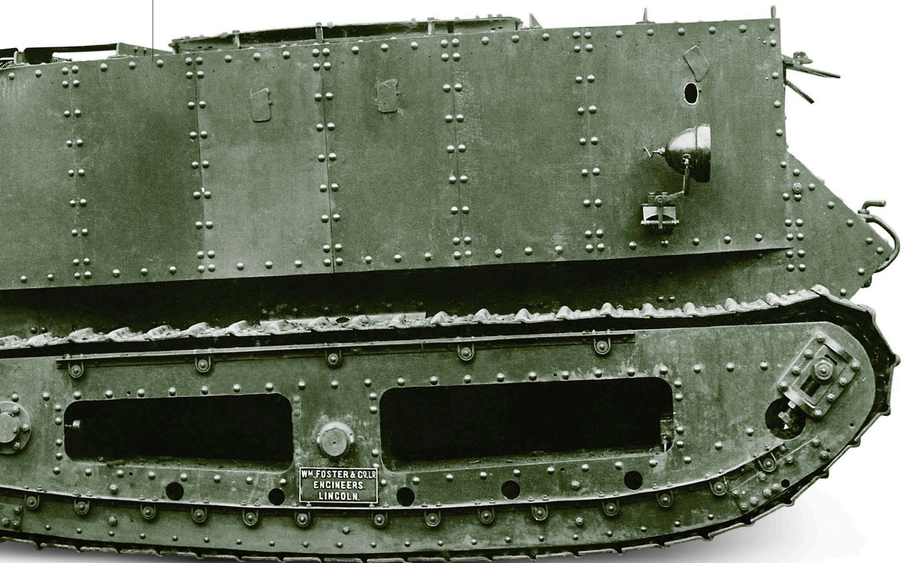
Riveted armor
