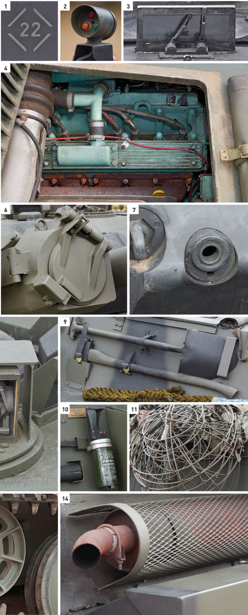
1. Insignia 2. Maneuvering light 3. Driver's periscope 4. Engine bay 5. Smoke grenade dischargers 6. Infrared light casing 7. Coaxial machine gun 8. Commander's periscope with wiper blade 9. Tools stowed on hull 10. Fire extinguisher 11. Camouflage netting basket 12. Cable drum 13. Track and idler wheel 14. Exhaust
