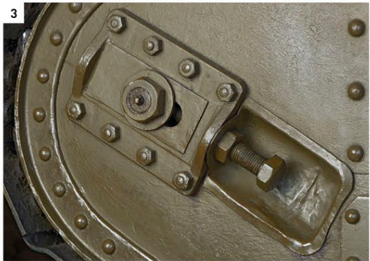
1. Tactical number 2. Driver’s vision port (closed) 3. Track tensioner 4. Male sponson with 6-pounder gun 5. Sponson ball machine gun mount (without gun) 6. Location of final drive 7. Track plates 8. Ventilation louvers 9. Rear escape hatch 10. Towing eye
