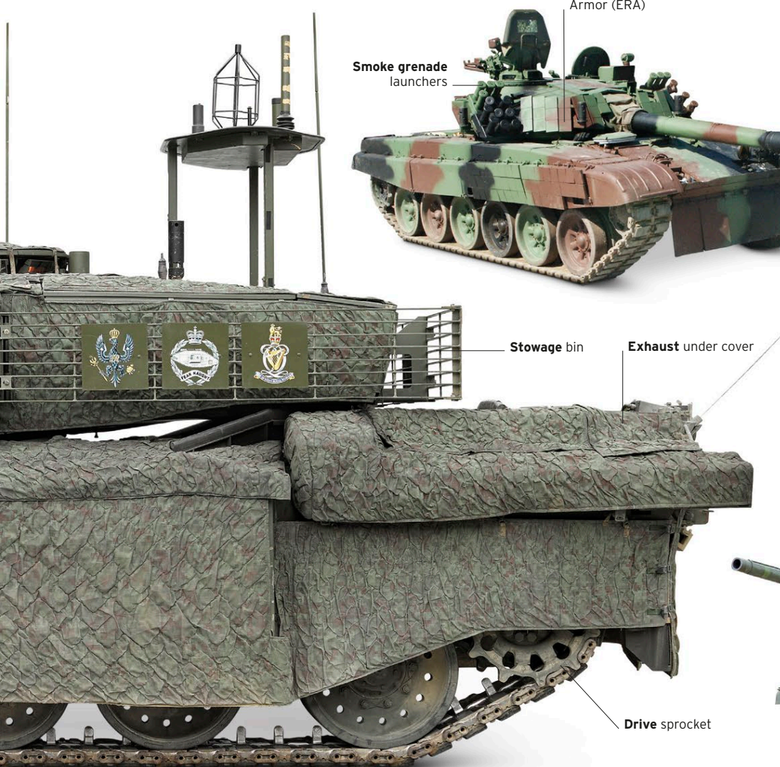
Explosive Reactive Armor (ERA)
