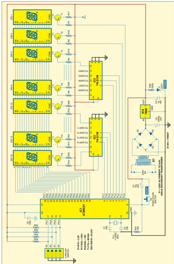
Fig. 1: Circuit for microcontroller-based moving-message display
