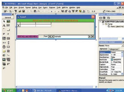
Screenshot 5: Form design of alert message utility program
